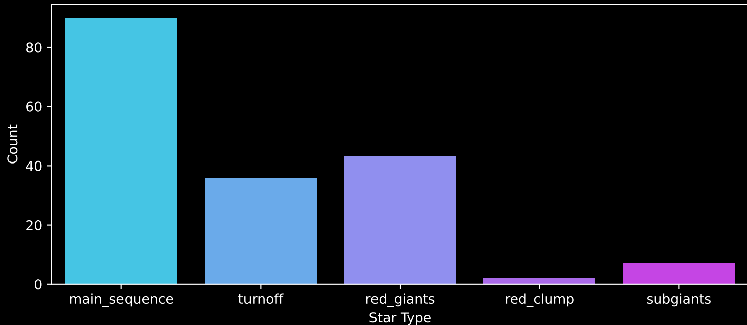
APOGEE DR17 Field: [233+36_MGA] Count plot of Star Type
