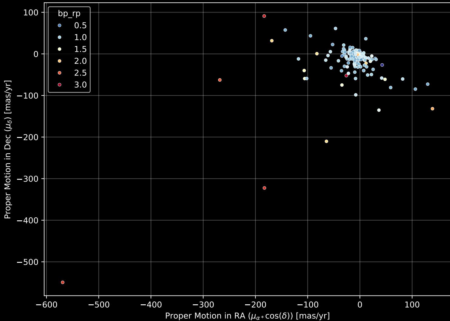
APOGEE DR17 Field: [233+36_MGA] Proper Motion Diagram (n= 178)
