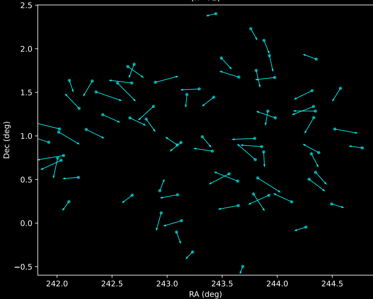
APOGEE DR17 Noise Stream Proper Motion Vectors (n=72)
