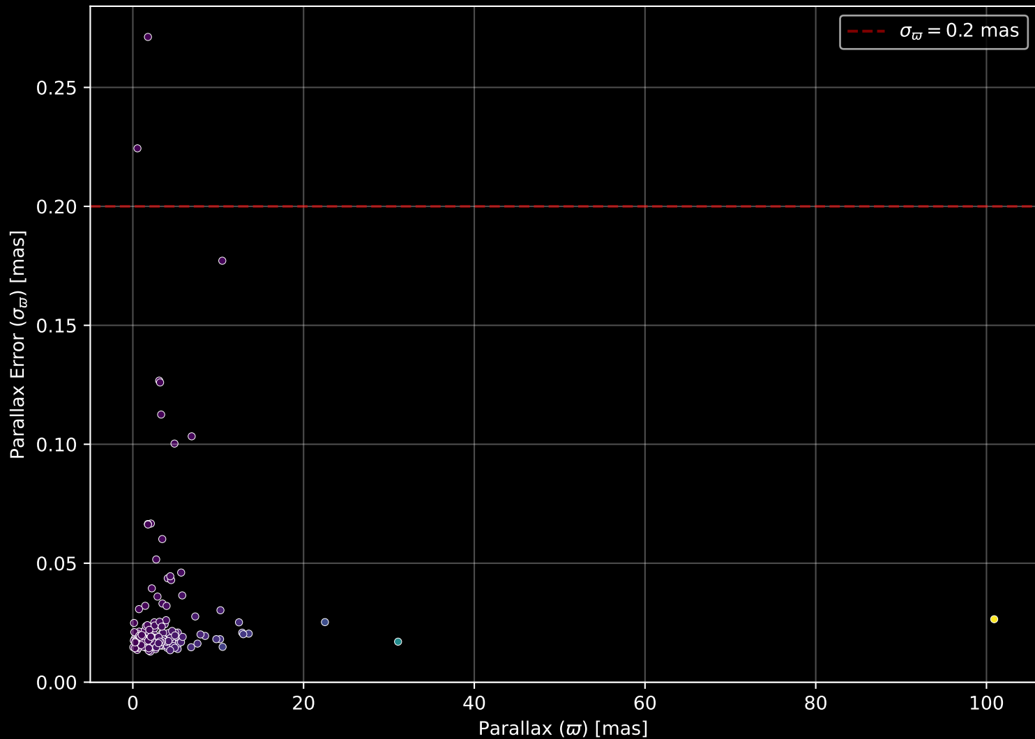
APOGEE DR17 Field: [233+36_MGA] Parallax Quality (n= 178)
