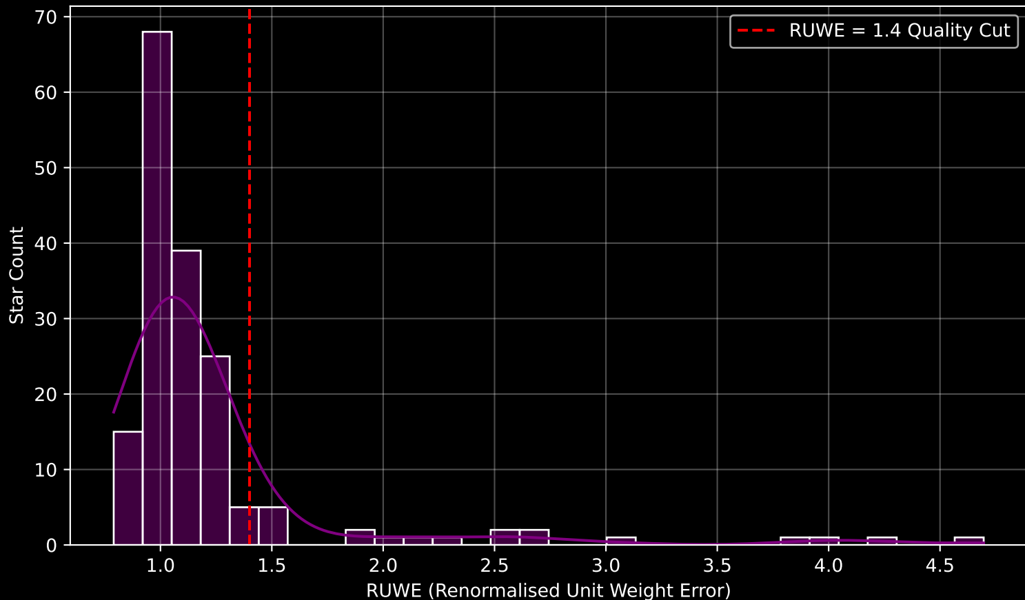
GAPOGEE DR17 Field [233+36_MGA] RUWE Distribution (n= 171)
