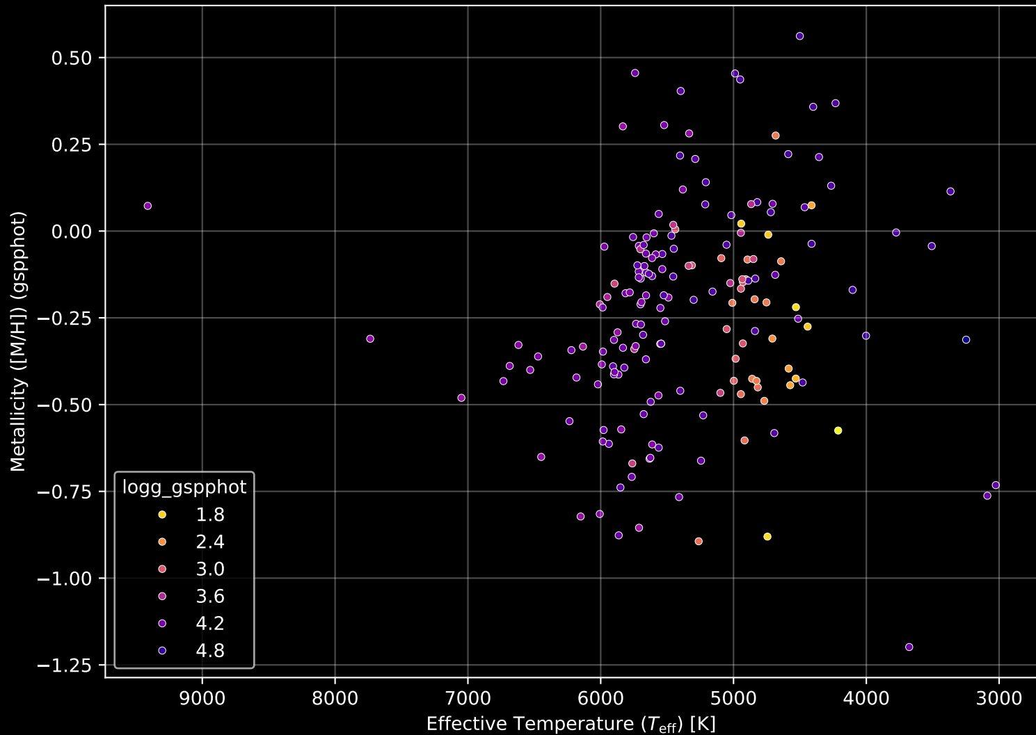
APOGEE DR17 Field: [233+36_MGA] Stellar Population Parameters (n= 178)
